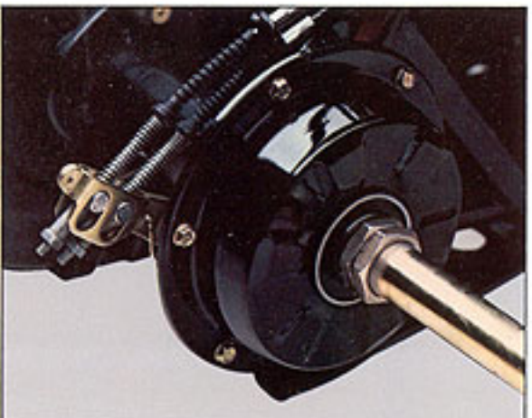
6. Fully enclosed rear drum brake.
